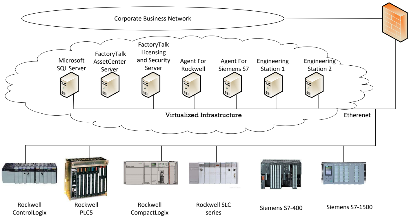
Figure 1: AssetCentre Architecture
